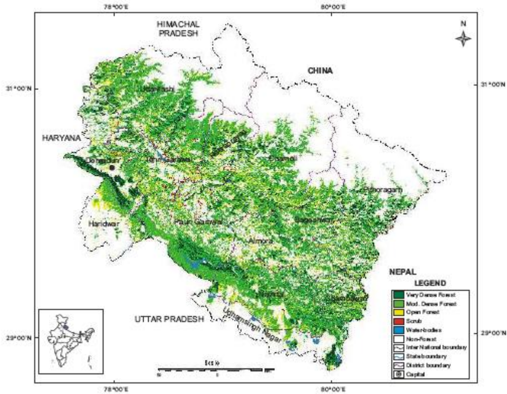
Fig 9.28 Forest Cover Map of Uttarakhand
