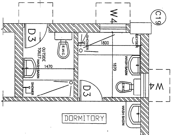
DORMITORY TOILET GROUND FLOOR
