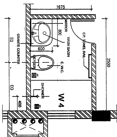
ATTACHED TOILET GROUND FLOOR
