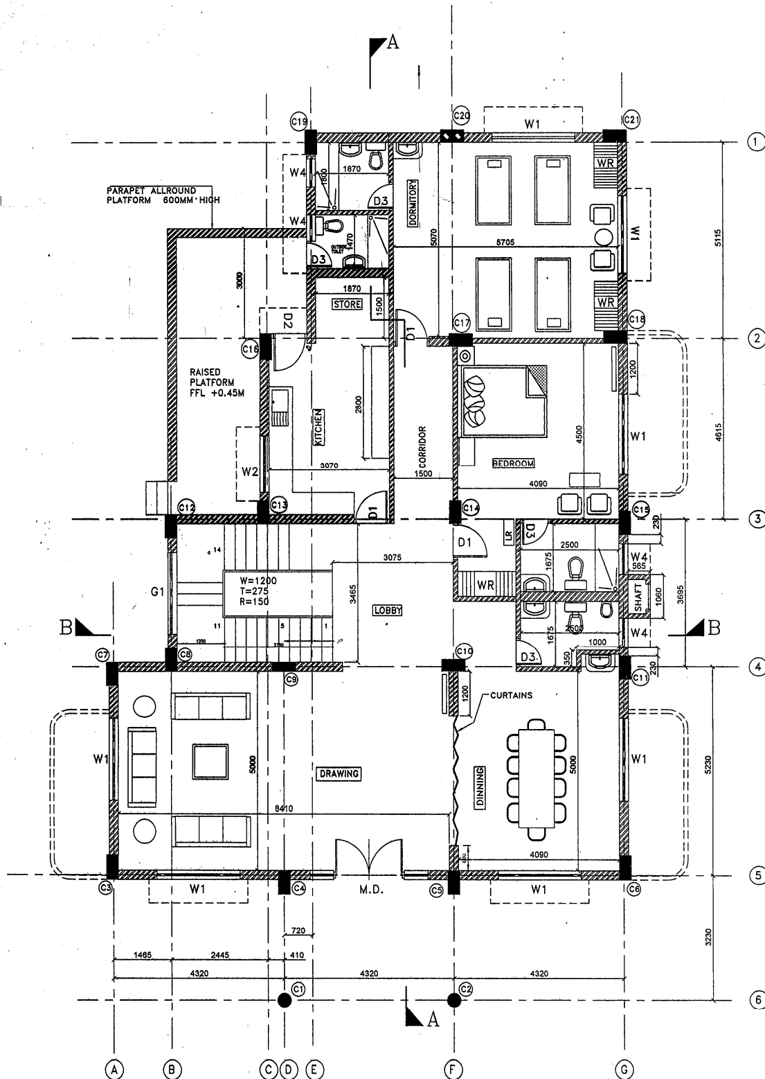
TRANSIT CAMP- GROUND FLOOR
