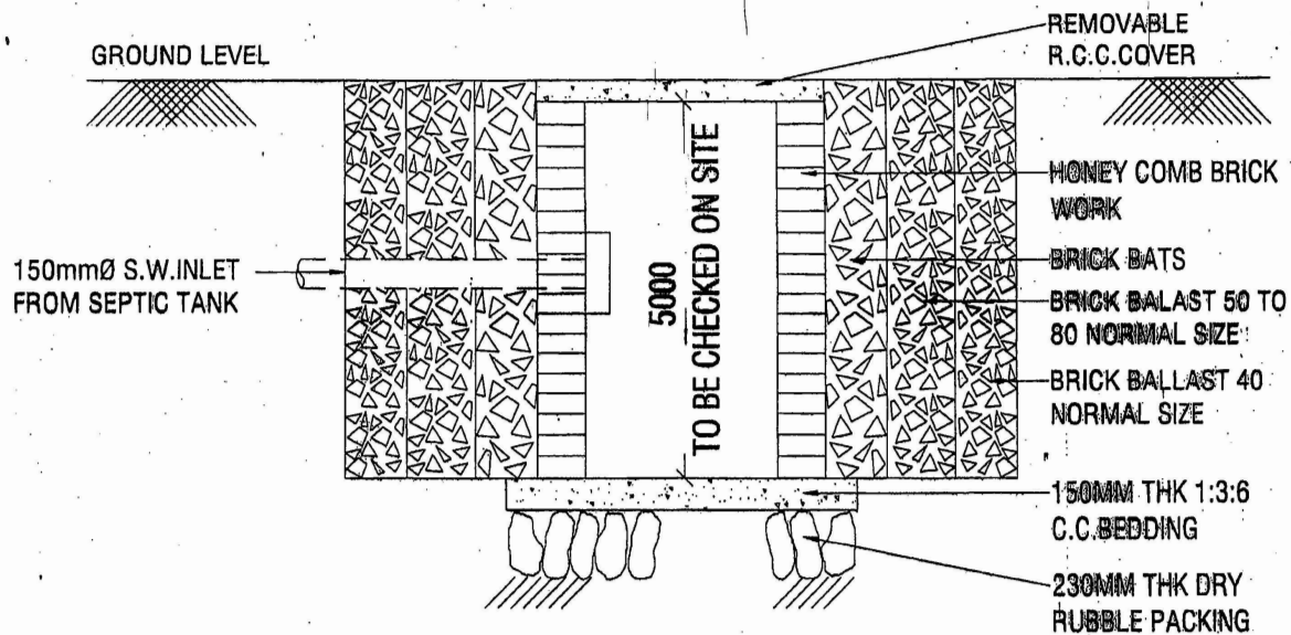
SECTION AT Z-Z'
