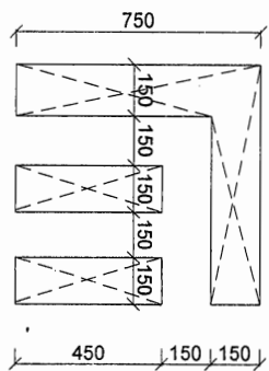
MUMTY PARAPET CUT-OUT DETAIL TYP.
