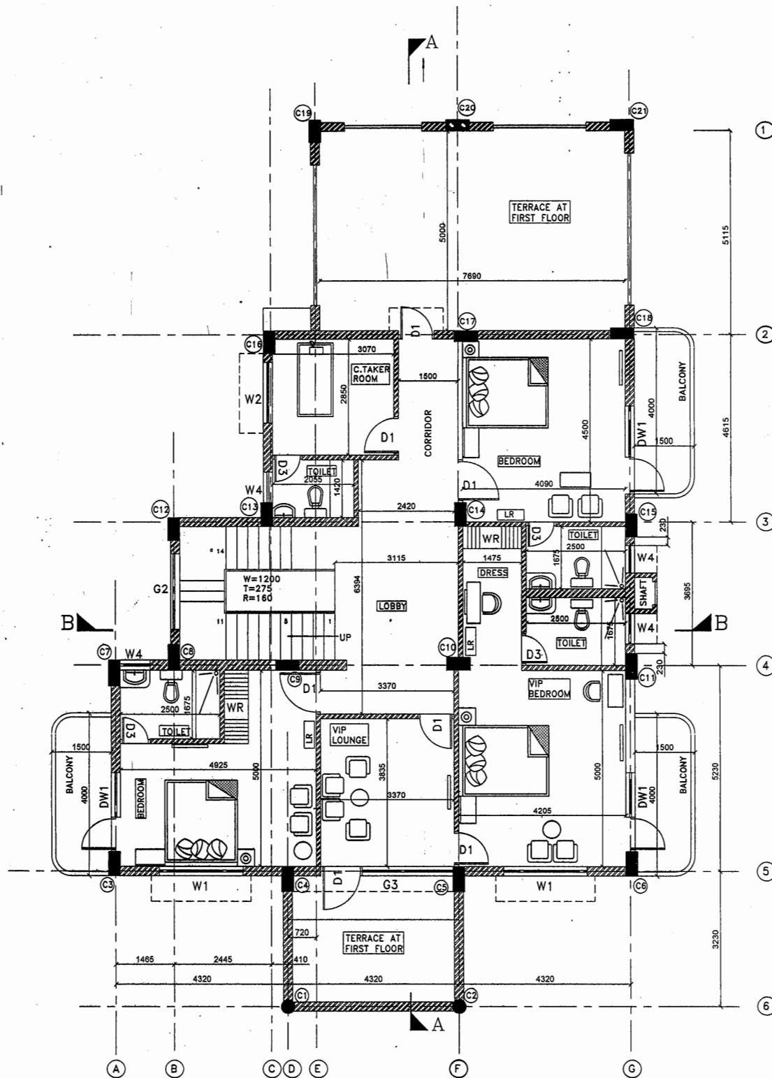
TRANSIT CAMP- FIRST FLOOR
