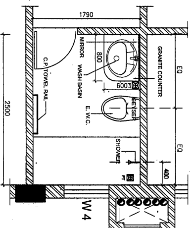
ATTACHED TOILET FIRST FLOOR
