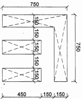
MUMTY PARAPET CUT-OUT DETAIL TYP.
