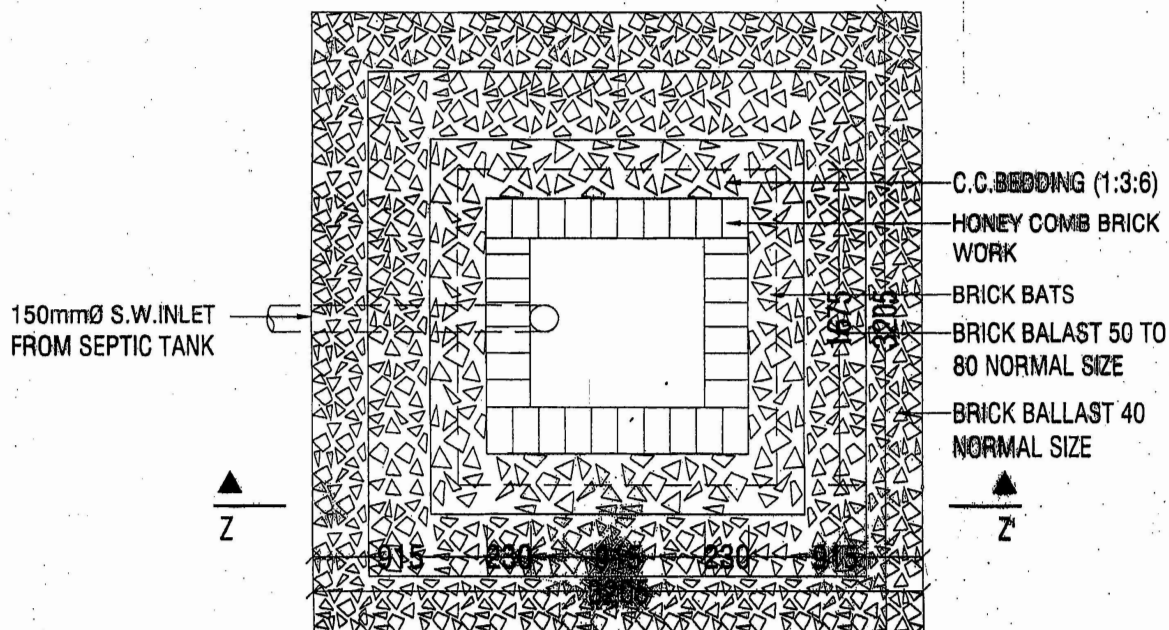
PLAN-SOAK PIT
