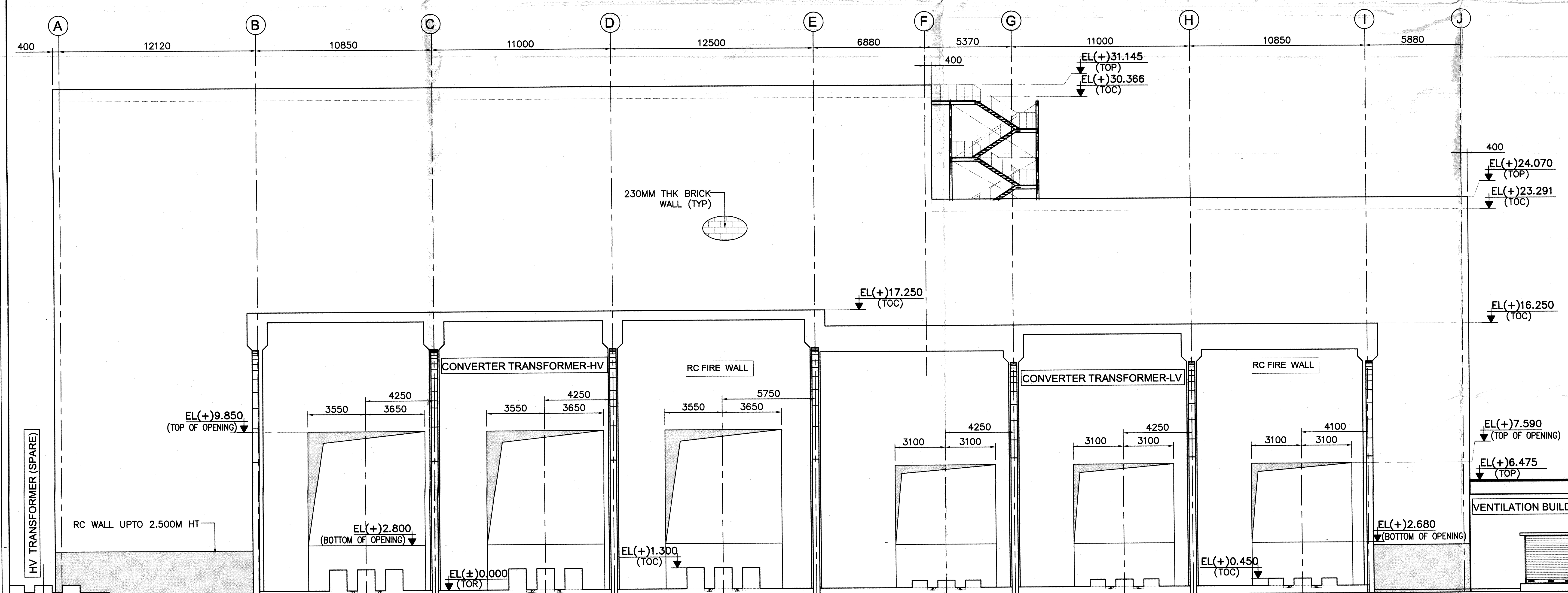
ELEVATION VIEW - A (SCALE 1:150)
